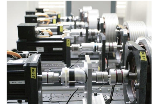
Motor load life test equipment
